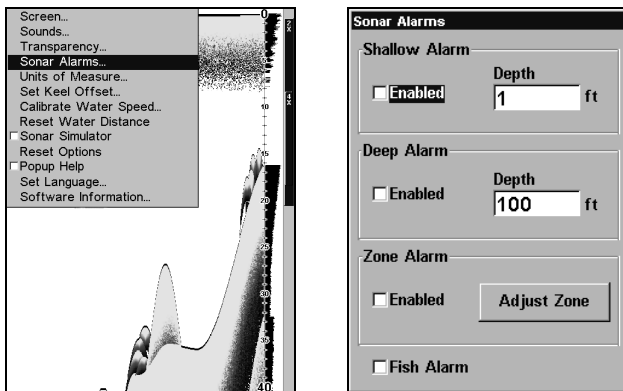
Main Menu (left) with Sonar Alarms highlighted. The Sonar Alarms menu is shown at right.
